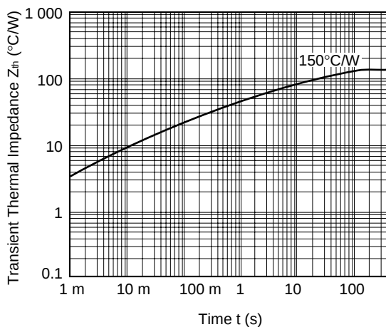
Fig. 10 Z_{th} CHARACTERISTIC
