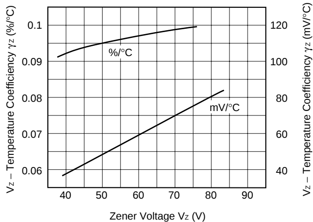
Fig. 6 \gamma_Z - V_Z CHARACTERISTIC
