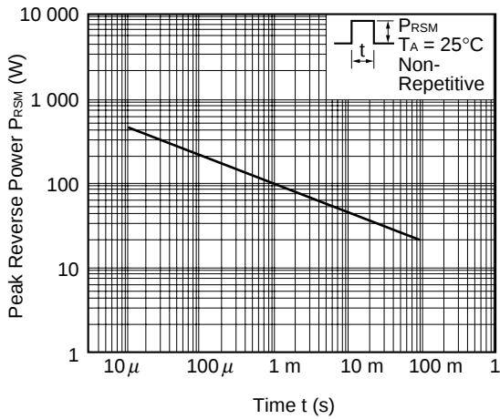
Fig. 9 P_{RSM} RATING
