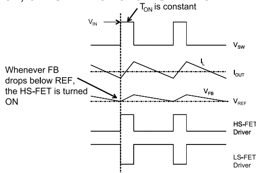
Figure 2—PWM Operation
