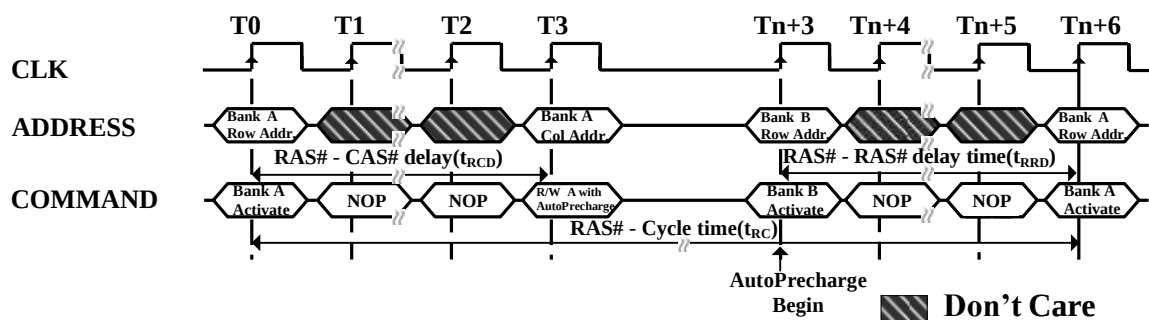
Figure 3. BankActivate Command Cycle (Burst Length = n, CAS# Latency = 3)
