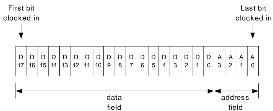
Figure 3. Serial Word Format
