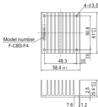
Fig.5 F-CBS-F4 external view
