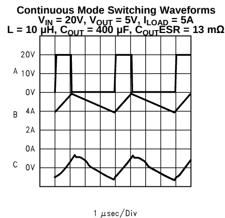
Figure 15. Horizontal Time Base: 1 \mu\text{s}/\text{div}
