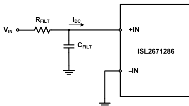
FIGURE 31. INPUT FILTERING
