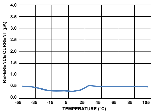
FIGURE 7. REFERENCE CURRENT vs TEMPERATURE
