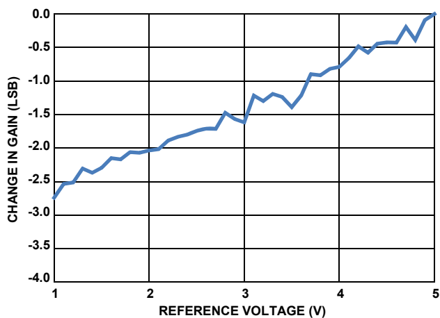
FIGURE 11. CHANGE IN GAIN vs REFERENCE VOLTAGE
