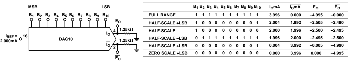
Figure 11. Basic Unipolar Negative Operation
