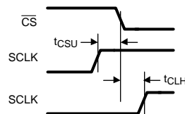
Figure 4. SCLK and \overline{\text{CS}} Timing Parameters
