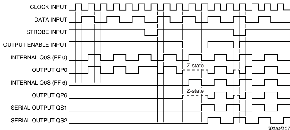
Fig 5. Timing diagram
