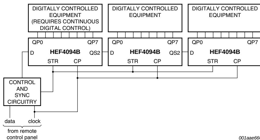
Fig 11. Remote control holding register
