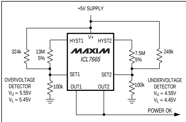
Figure 6. Fault Monitor for a Single Supply
