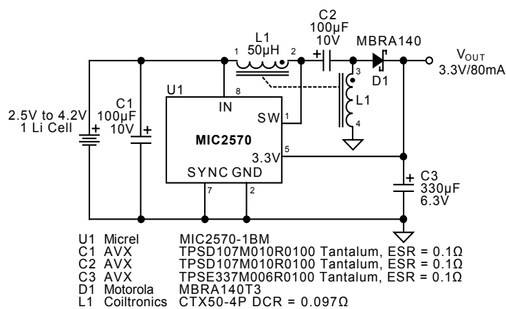
Example 4. Single Cell Lithium to 3.3V/80mA Regulator
