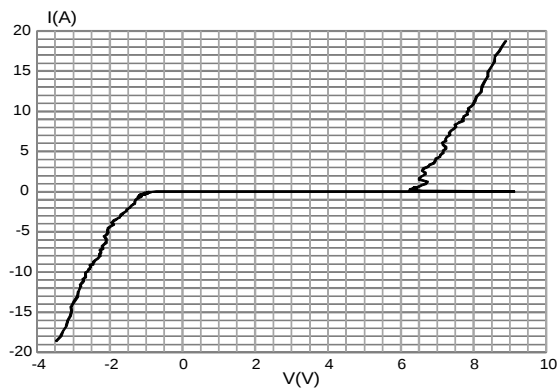
Figure 7: TLP characteristic
