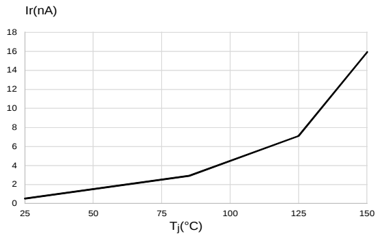
Figure 3: Leakage current versus junction temperature (typical values)
