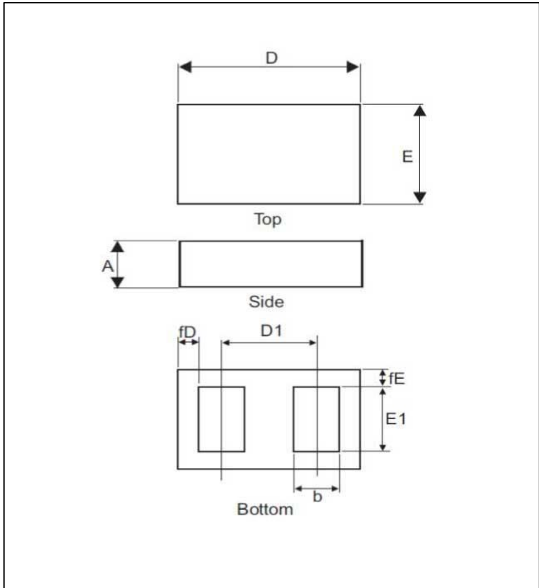
Figure 9: 0201 package outline
