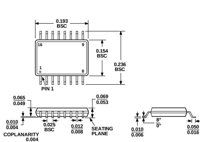
Figure 40. 16-Lead Shrink Small Outline Package [QSOP] (RQ-16)
