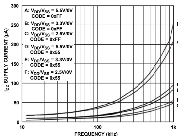
Figure 18. Supply Current vs. Frequency
