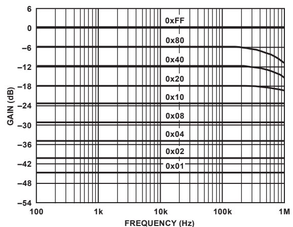
Figure 19. AD5242 10 kΩ Gain vs. Frequency vs. Code
