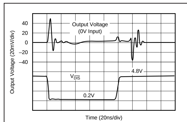
FIGURE 8. Disable/Enable Glitch.
