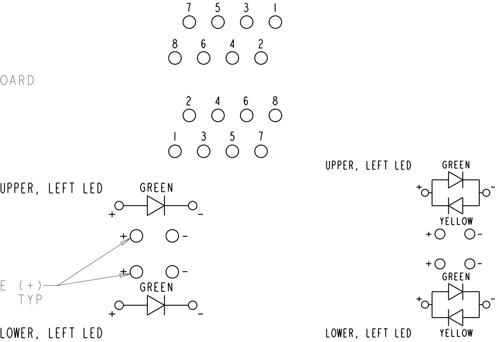
6368116-1, -2 LED SCHEMATIC
