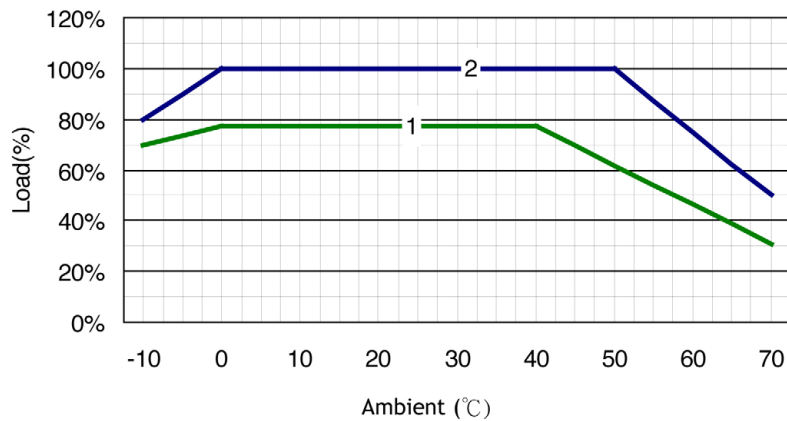
Open-Frame (PMK130S-xx) :
