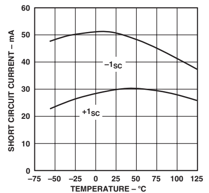
TPC 18. Short-Circuit Current vs. Temperature @ \pm 15 V
