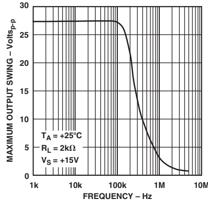
TPC 11. OP183/OP283 Maximum Output Swing vs. Frequency @ \pm 15 V
