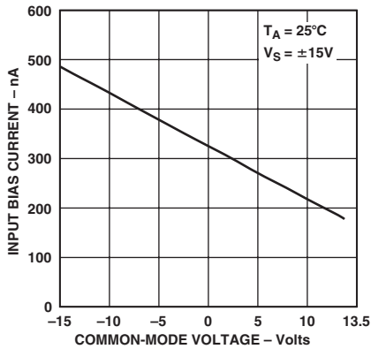
TPC 13. Input Bias Current vs. Common-Mode Voltage
