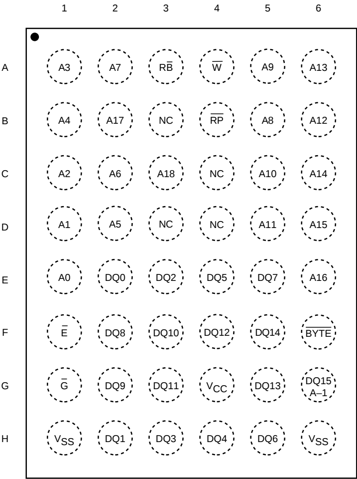
Figure 5. TFBGA Connections (Top view through package)
