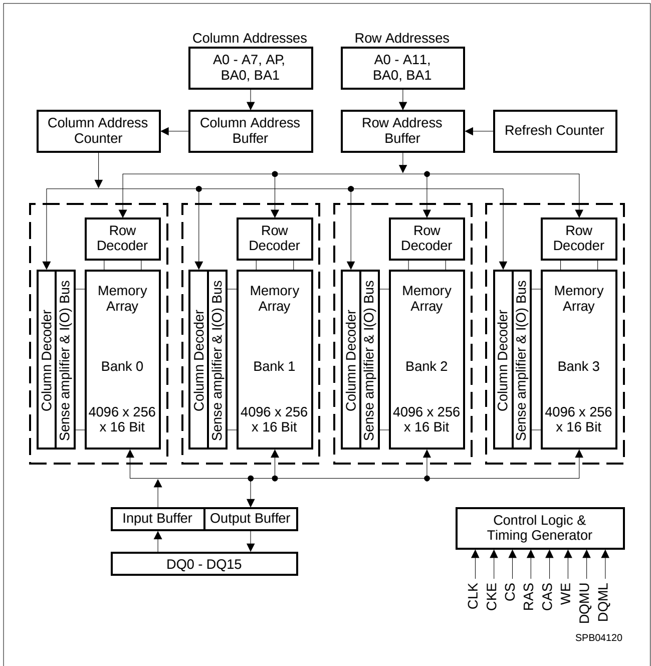
Block Diagram: 4 Bank \times 1M \times 16 SDRAM
