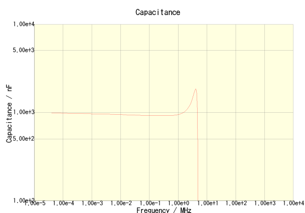
CKCA43X5R0J105M100AA
