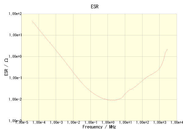
CKCA43X5R0J105M100AA
