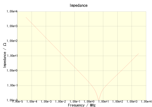
CKCA43X5R0J105M100AA
