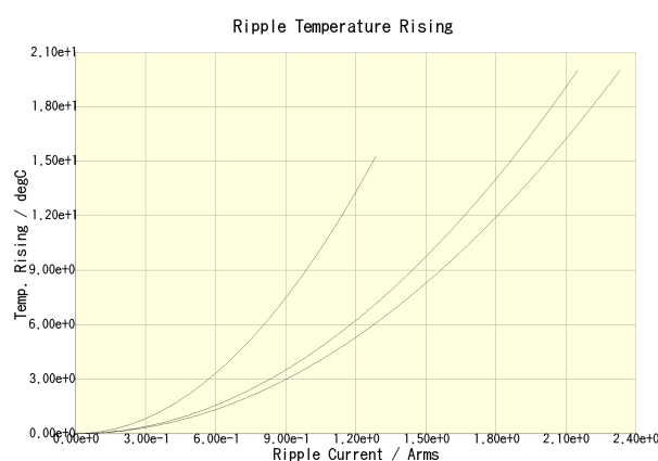
CKCA43X5R0J105M100AA(100kHz) CKCA43X5R0J105M100AA(500kHz) CKCA43X5R0J105M100AA(1MHz)
