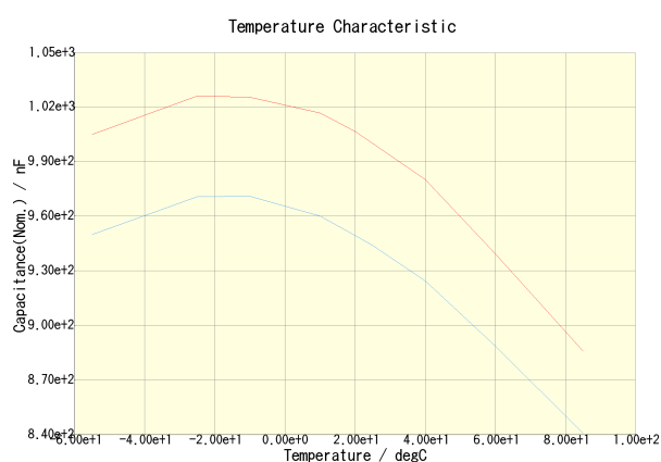
CKCA43X5R0J105M100AA(DC Bias = 0V) CKCA43X5R0J105M100AA(DC Bias = 3.15V)
