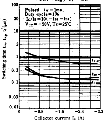
t_{on}, t_{sg}, t_f - I_C
