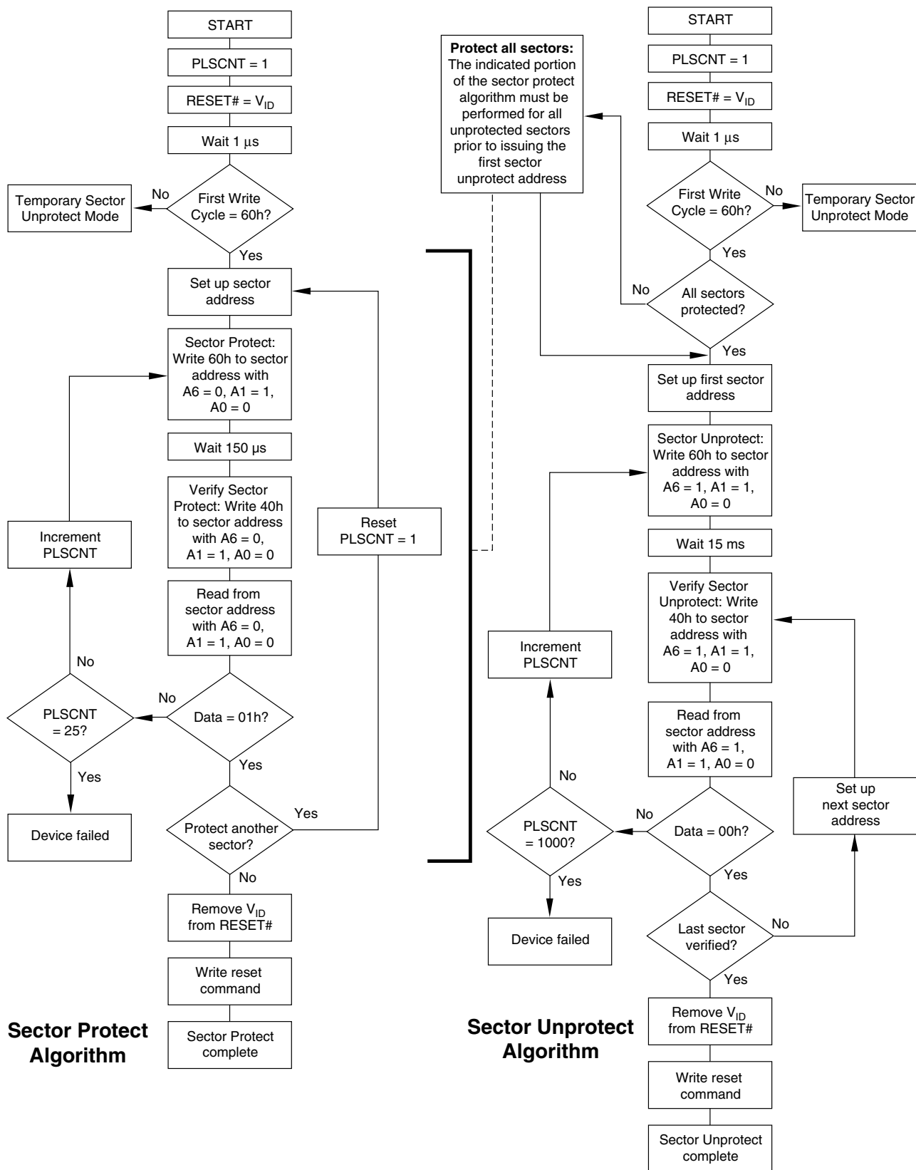
Figure 2. In-System Sector/Sector Block Protection and Unprotection Algorithms
