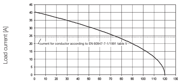
HDC-S4-SAS/BAS H07V-K2,5 Ambient temperature [°C]
