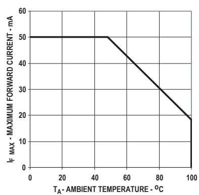
Figure 4. Forward current vs. ambient temperature
