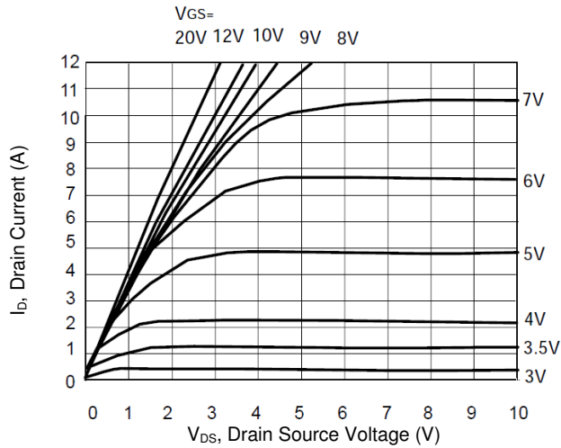
Figure 1. Saturation Characteristics
