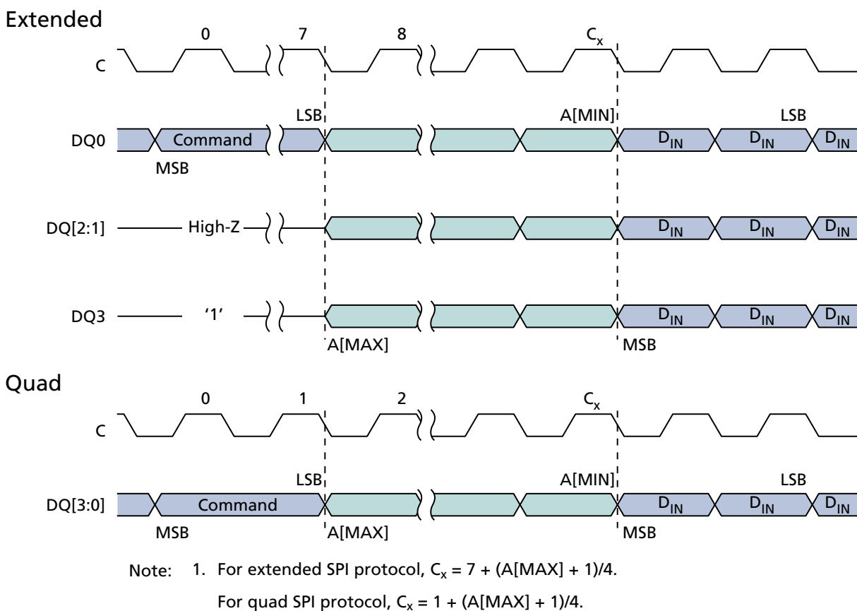
Figure 30: EXTENDED QUAD INPUT FAST PROGRAM Command
