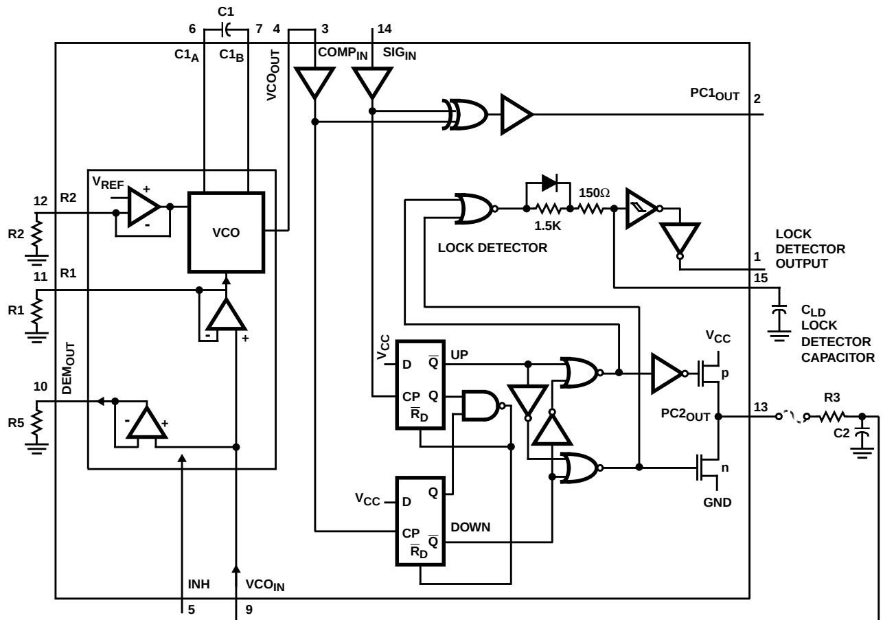
FIGURE 1. LOGIC DIAGRAM
