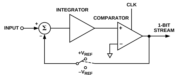
Figure 6. AD7741/AD7742 Modulator Loop
