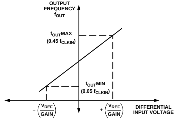
Figure 5. AD7742 Transfer Characteristic for Bipolar Differential Input Range: -V_{REF}/\text{Gain} to +V_{REF}/\text{Gain} ; the common-mode range must be between +0.5 V and V_{DD} - 1.75 V. UNI/BIP pin tied to GND.
