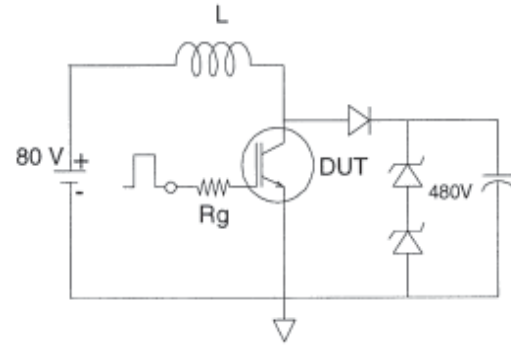
Fig.C.T.2 - RBSOA Circuit
