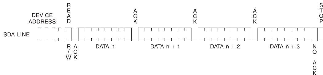
Figure 12. Sequential Read
