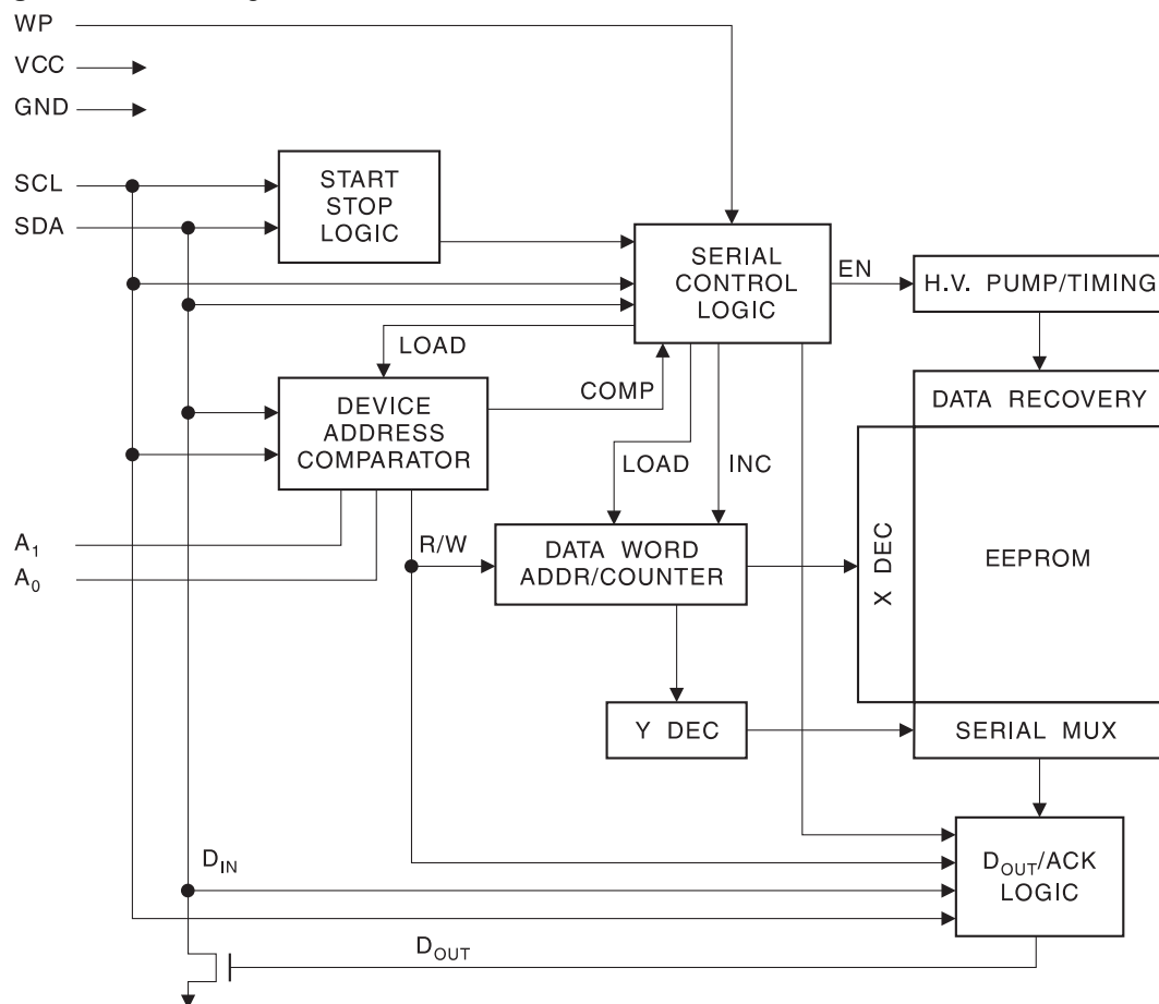
Figure 1. Block Diagram
