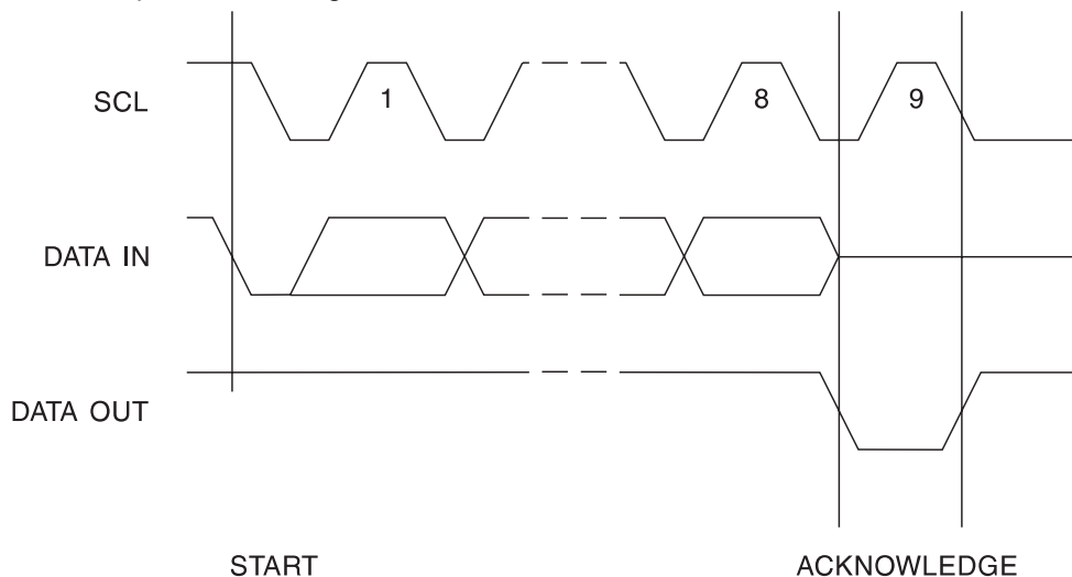
Figure 6. Output Acknowledge
