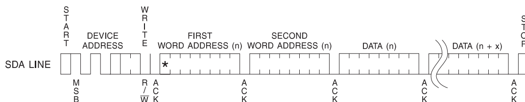
Figure 9. Page Write
