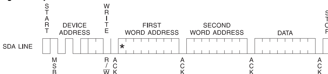
Figure 8. Byte Write
