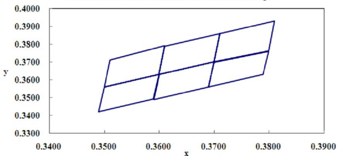
Lumimicro Ltd. Yellowsh White C.I.E Graph
