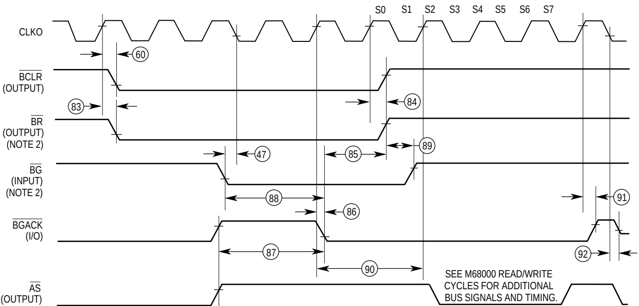
Figure 6-7. DMA Timing Diagram (SDMA)
