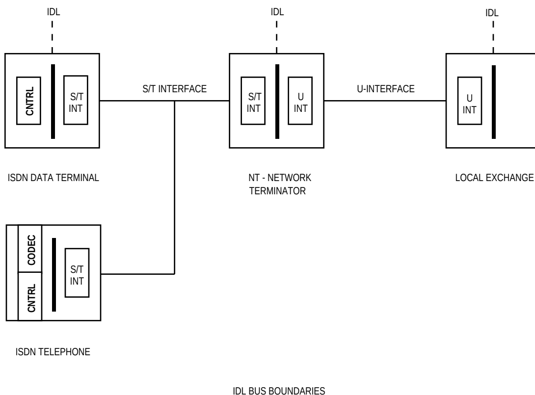
Figure D-12. IDL Bus Boundaries
