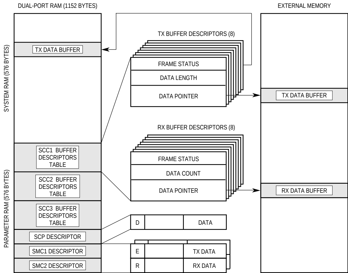
Figure 4-15. Memory Structure
