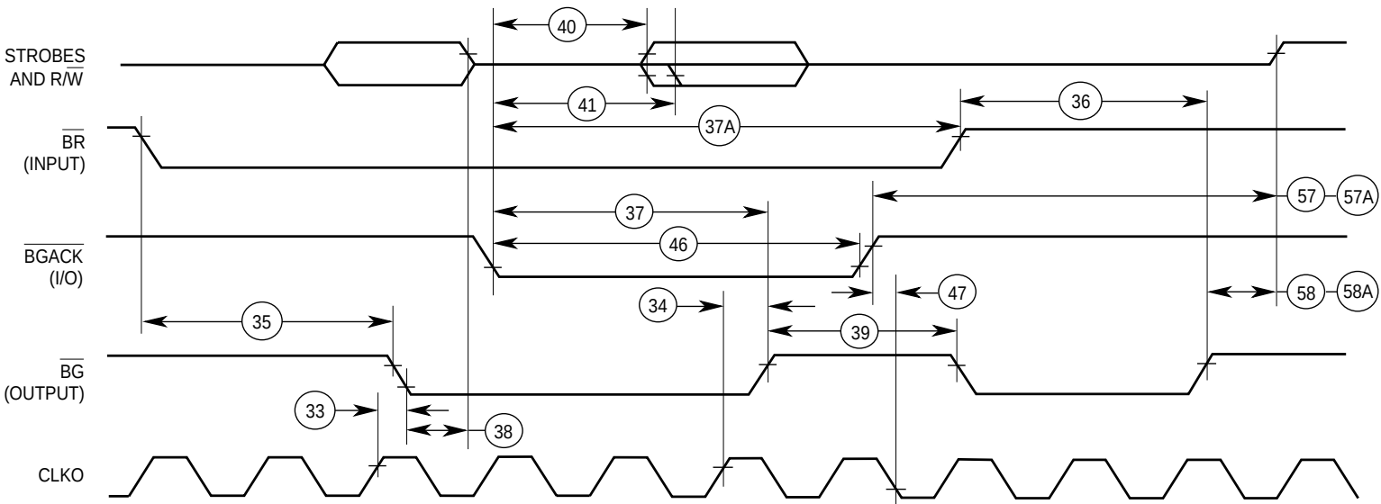
Figure 6-5. Bus Arbitration Timing Diagram
