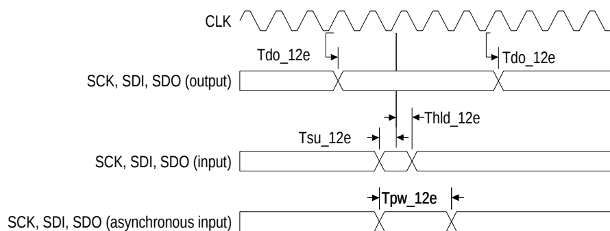
Figure 18 SPI AC Timing Waveform — Bit I/O Mode
