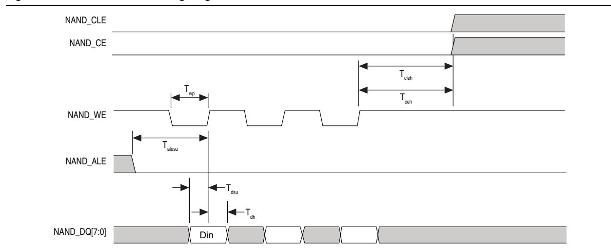
Figure 18. NAND Data Write Timing Diagram
