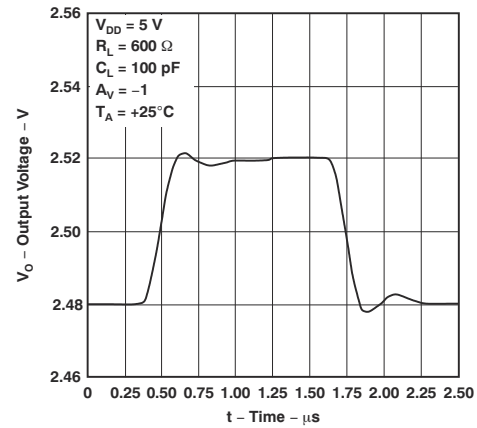
Figure 6-28. Voltage-Follower Small-Signal Pulse Response
