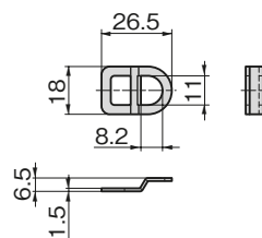
適用ハンドル断面寸法(最大) Applicable handle cross section dimension (max.) 推奨製品 Recommended products FA-1825N-2
