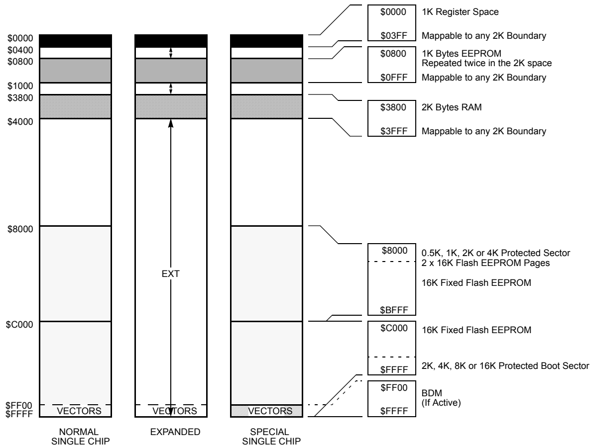
Figure 6 MC9S12K32 User Configurable Memory Map
