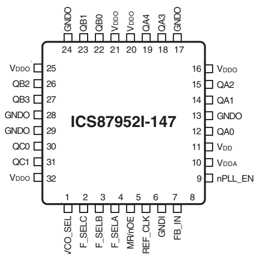
32-Lead LQFP
