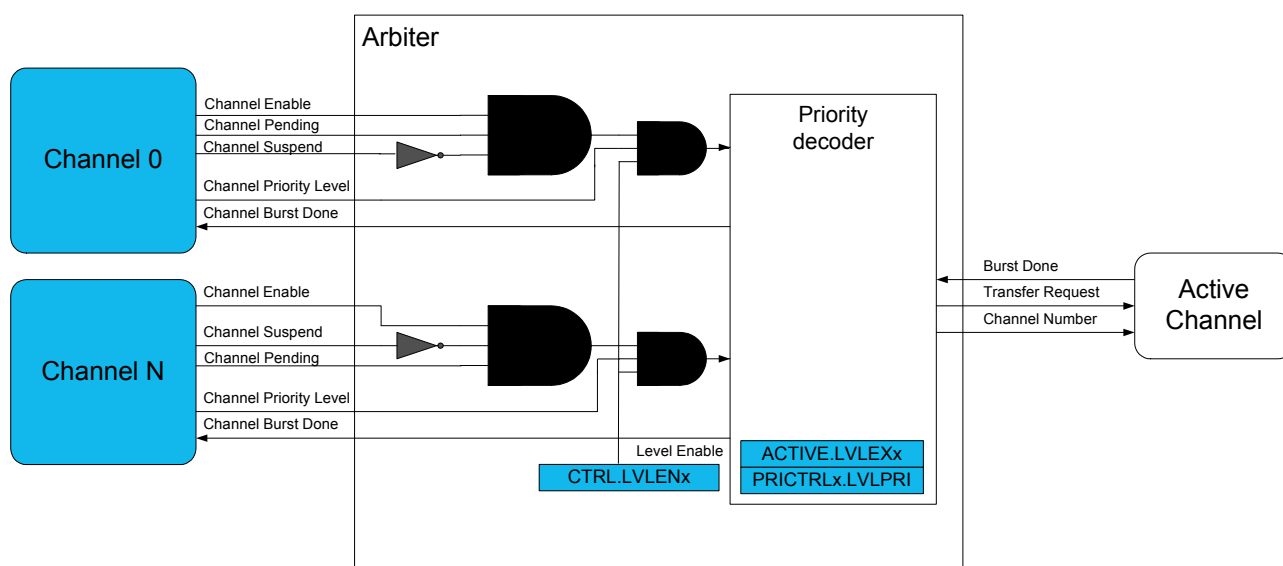
Figure 18-4. Arbiter Overview
