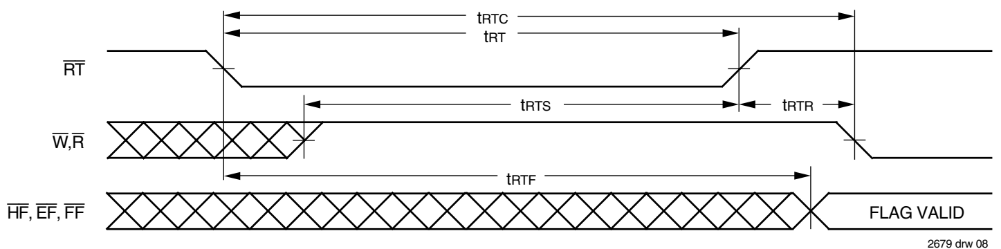
Figure 6. Retransmit
