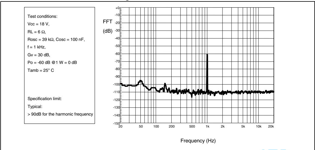
Figure 10. FFT -60 dB
