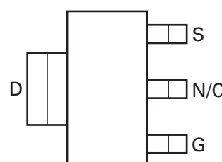
Pinout - top view
