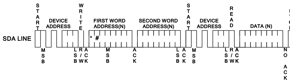
Figure 7: Random Read
