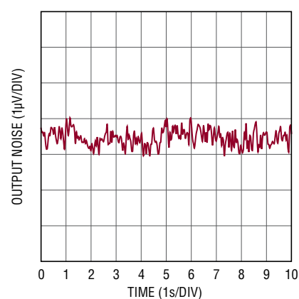
1.25V Output Noise 0.1Hz to 10Hz
