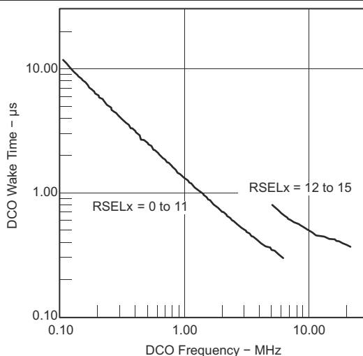
Figure 8-18. DCO Wake-up Time From LPM3 vs DCO Frequency
