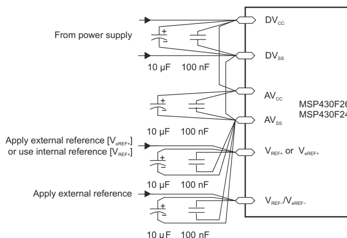
Figure 8-39. Supply Voltage and Reference Voltage Design V_{REF-}/V_{eREF-} . External Supply
