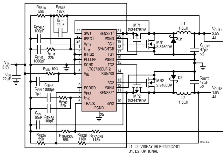
2-Phase, 750kHz, Dual Output Synchronous DC/DC Converter
