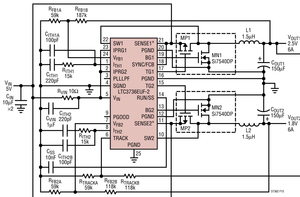
Figure 15. 2-Phase, 550kHz, Dual Output Synchronous DC/DC Converter
