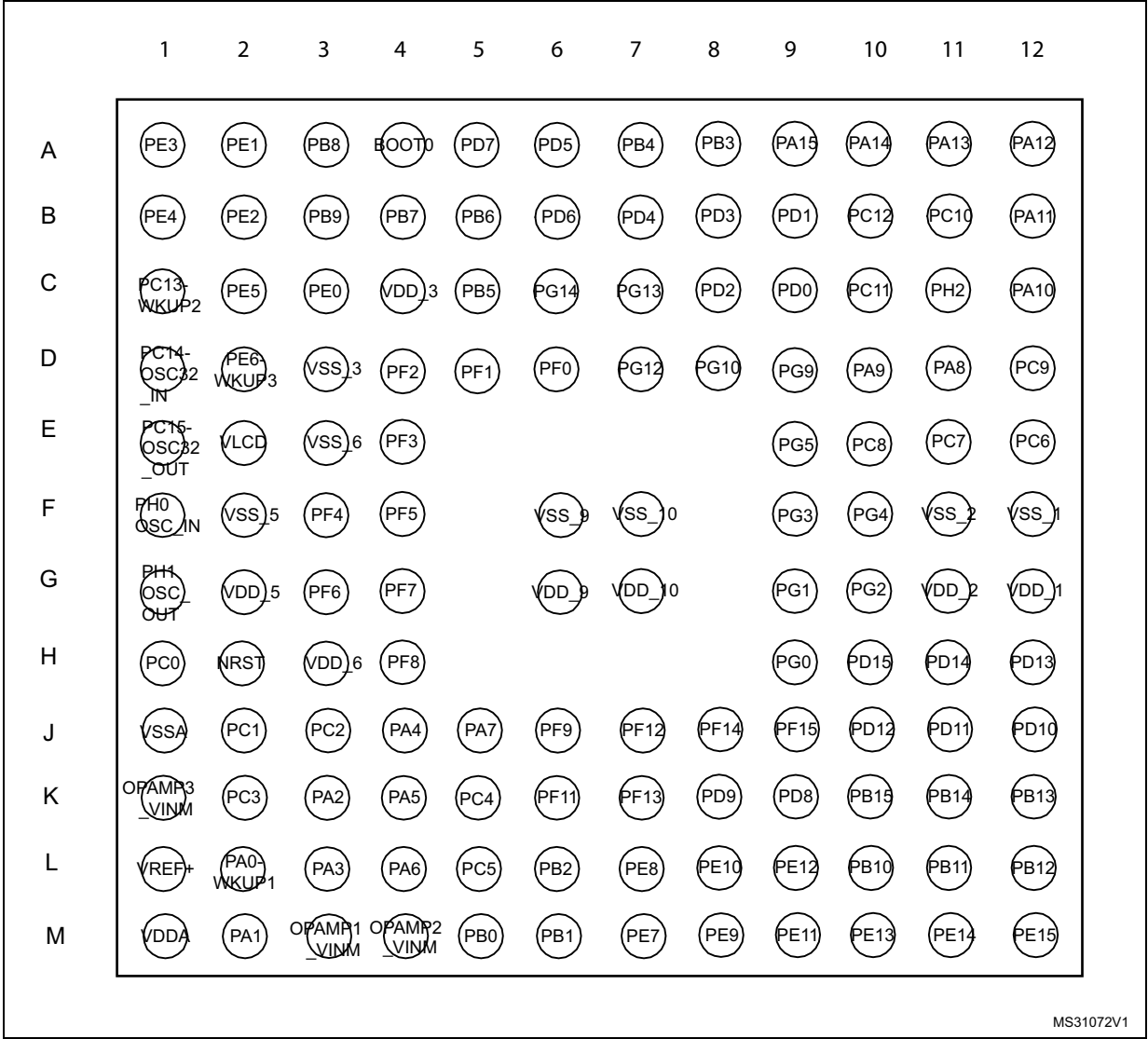
Figure 6. STM32L15xQC UFBGA132 ballout
