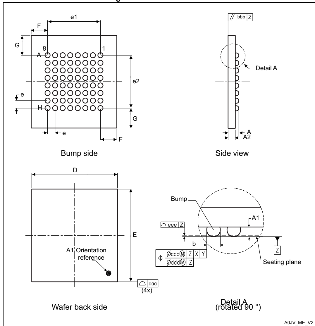
Figure 34. WLCSP64 outline
