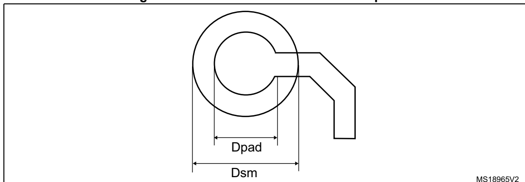
Figure 35. WLCSP64 recommended footprint
