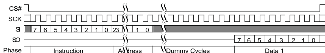
Figure 50. RSFDP Command Sequence
